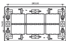
Cutout size— 253mm x 112mm Code No: 373015 20 module — 7.5" X 13"
