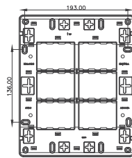
Cutout size— 152mm x 167mm Code No: 373014 18 module — 8.5" X 10.5"
