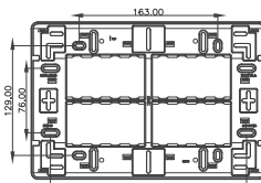
Cutout size— 196mm x 112mm Code No: 373013 16 module — 7.5" X 11"
