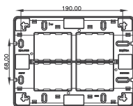
Cutout size— 151mm x 112mm Code No: 373012 12SQR module — 7" X 9"
