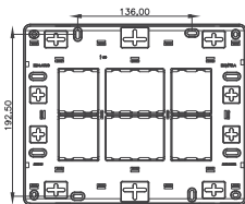
Cutout size— 186mm x 112mm Code No: 373011 14 module — 8.5" X 10.5"
