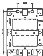
Cutout size— 130mm x 116mm Code No: 373019 10SQR module — 7" X 9"
